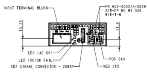
PSU Front View (24V & 48V UNITS)
