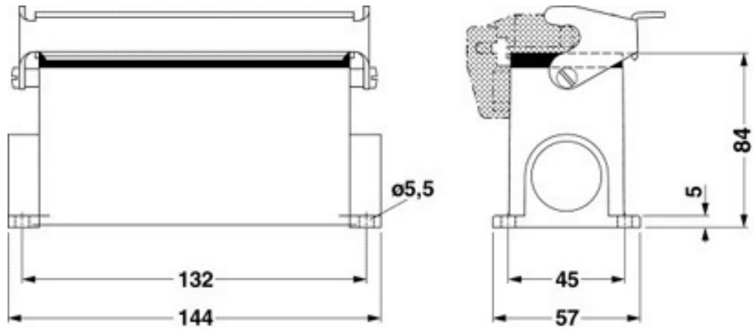
Dimensioned drawing
