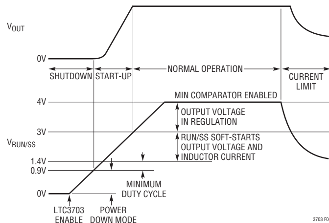
Figure 4. Soft-Start Operation in Start-Up and Current Limit
