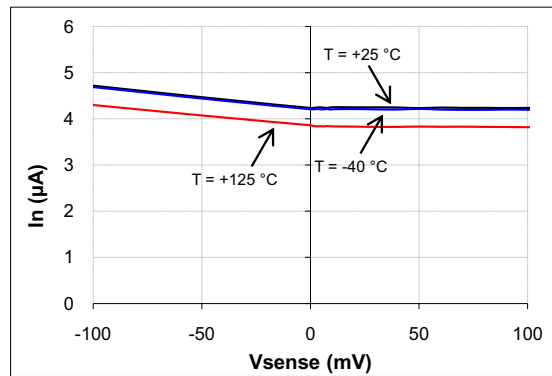
Figure 8. Vn pin input current vs. Vsense
