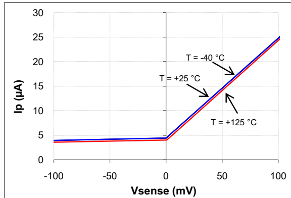
Figure 7. Vp pin input current vs. Vsense
