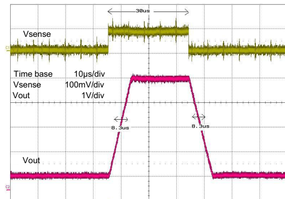
Figure 12. Step response
