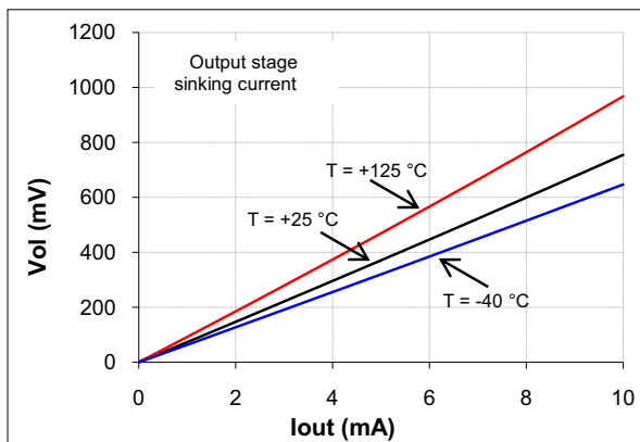
Figure 9. Output stage low-state saturation voltage vs. output current (Vsense = -1 V)
