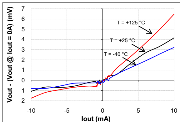
Figure 11. Output stage load regulation
