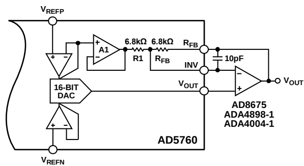
Figure 52. Output Amplifier in Gain of Two Configuration
