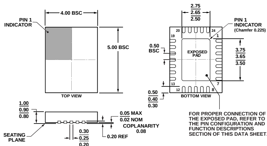
Figure 54. 24-Lead Lead Frame Chip Scale Package [LFCSP_VQ] 4 mm × 5 mm, Very Thin Quad (CP-24-5) Dimensions shown in millimeters
