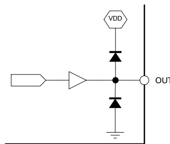
TYPE 4: DO, WDb, ERRb Push Pull Output
