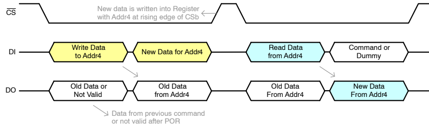
Figure 29. WRITE Operation Followed by a READ operation to verify
