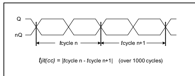
Figure 8: Cycle-to-Cycle Jitter
