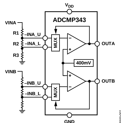
Figure 2. ADCMP343
