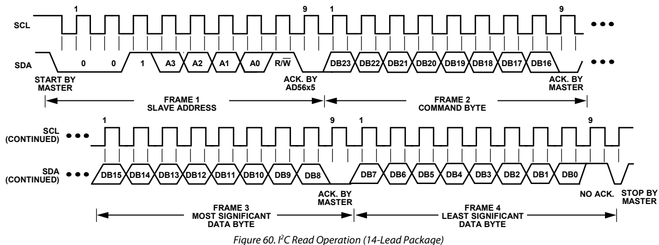
Figure 60. I 2 C Read Operation (14-Lead Package)
