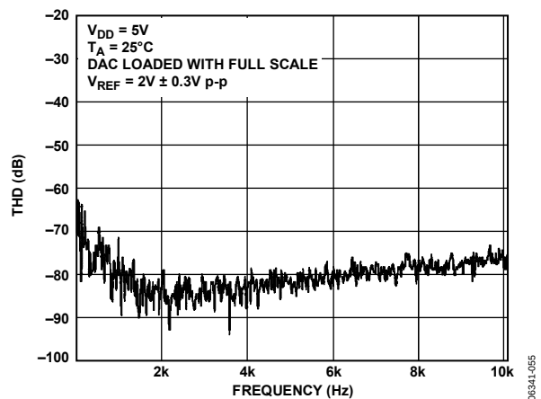
Figure 51. Total Harmonic Distortion
