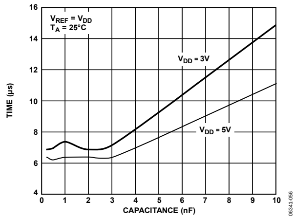
Figure 52. Settling Time vs. Capacitive Load
