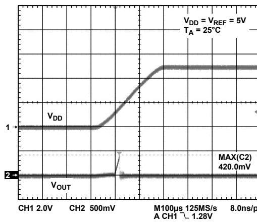
Figure 42. Power-On Reset to 0 V
