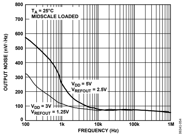
Figure 50. Noise Spectral Density, Internal Reference
