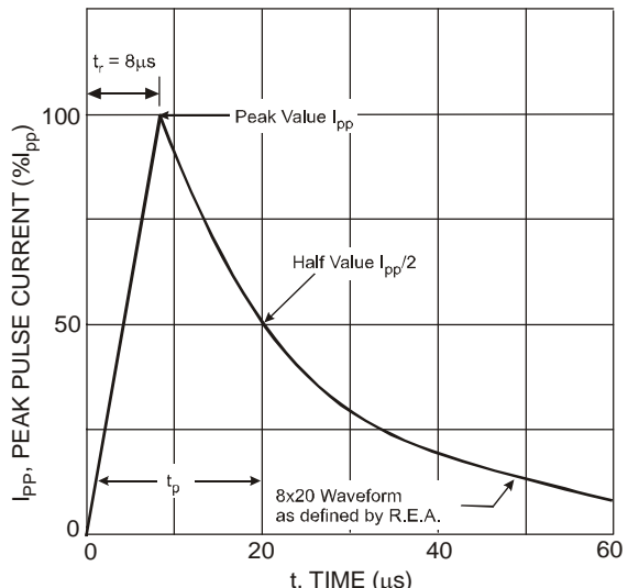
Fig. 2 Typical 8 x 20μs Pulse Waveform
