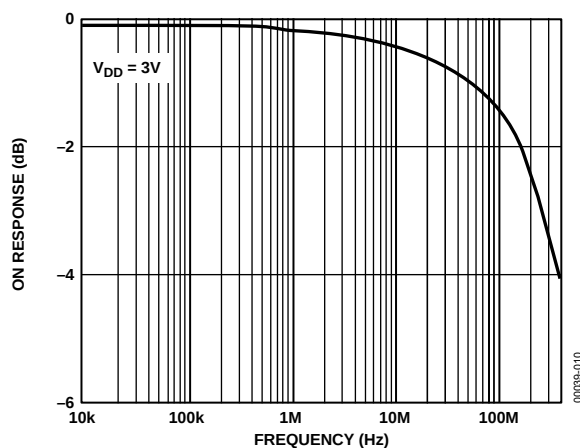
Figure 10. On Response vs. Frequency
