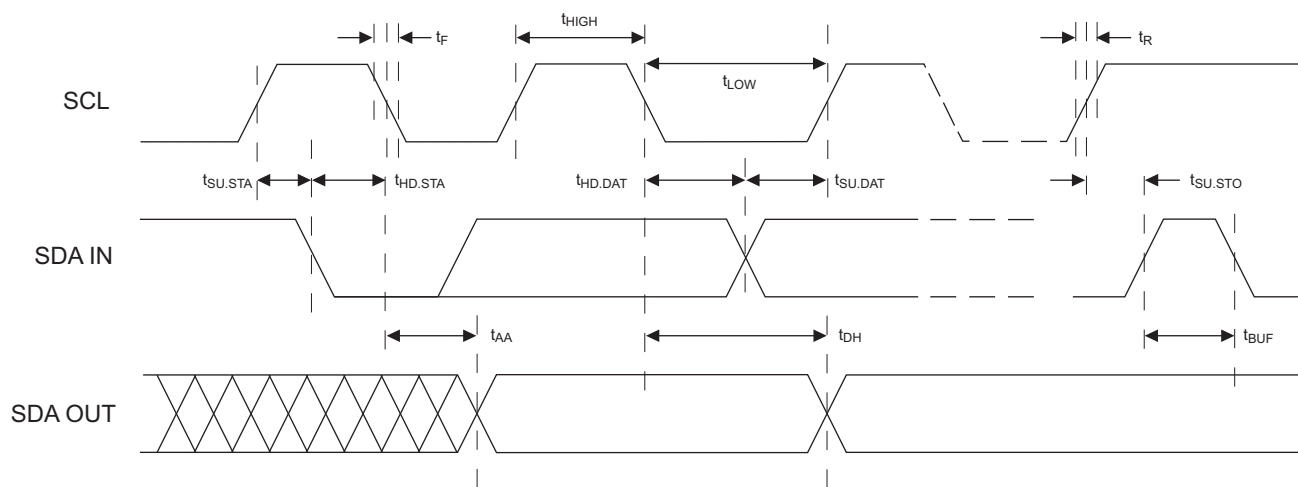
Figure 8-1. Bus Timing
