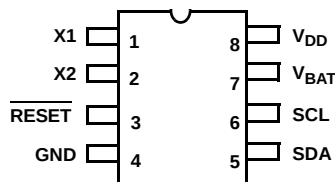
ISL12027 (8 LD SOIC) TOP VIEW
