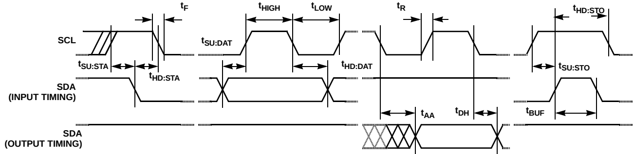
FIGURE 1. BUS TIMING
