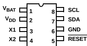
ISL12027 (8 LD TSSOP) TOP VIEW
