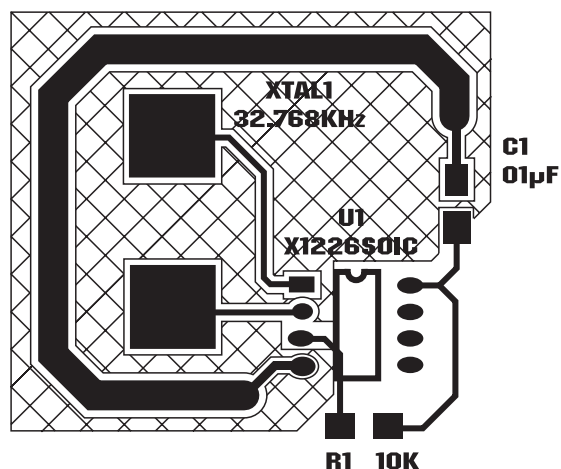
FIGURE 27. SUGGESTED LAYOUT FOR INTERSIL RTC IN SO-8
