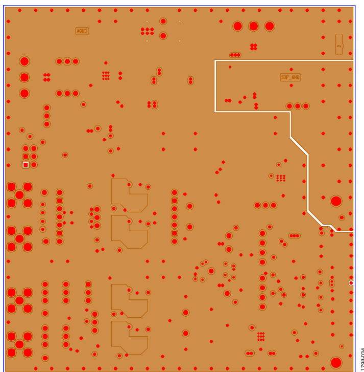
Figure 34. EVAL-AD7902SDZ Evaluation Board Layer 2—Ground
