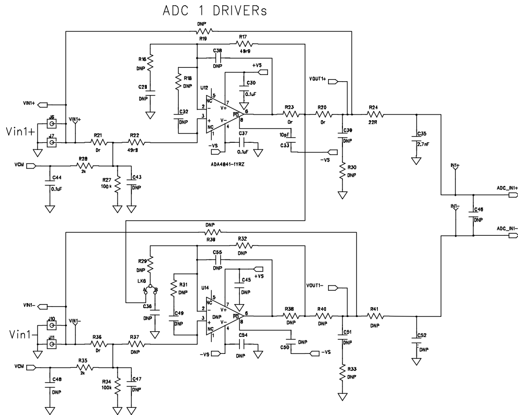
Figure 26. Schematic, Page 1
