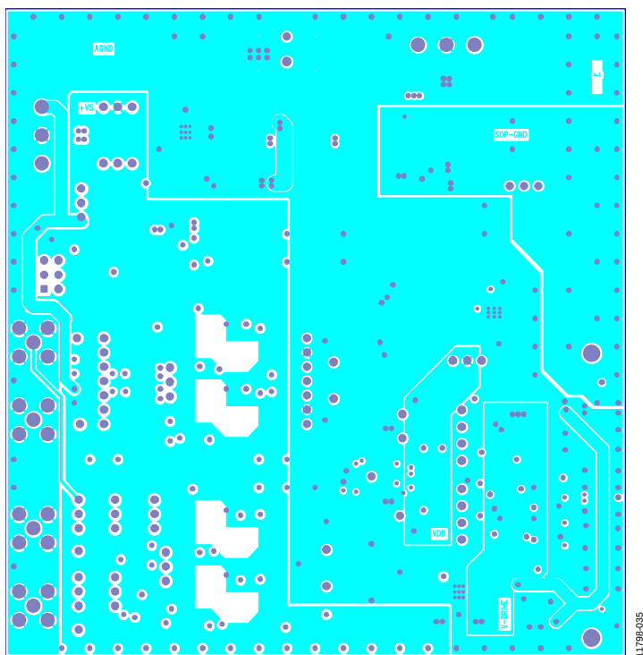
Figure 35. EVAL-AD7902SDZ Evaluation Board Layer 3—Power
