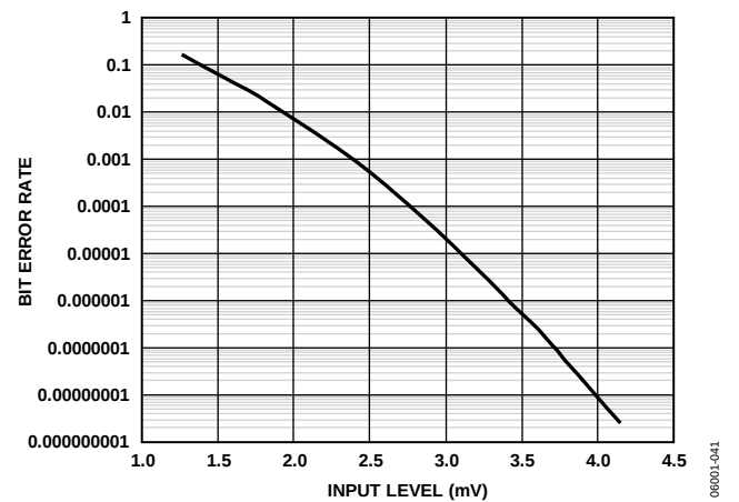
Figure 17. Bit Error Rate vs. Input Level
