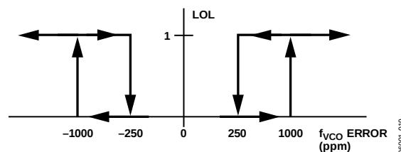
Figure 30. Transfer Function of LOL
