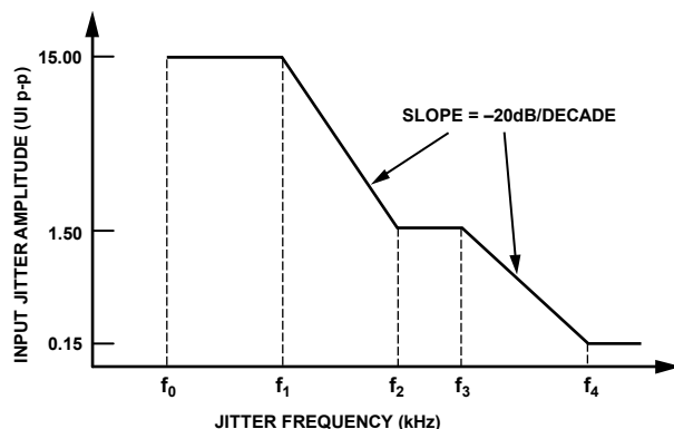
Figure 27. SONET Jitter Tolerance Mask
