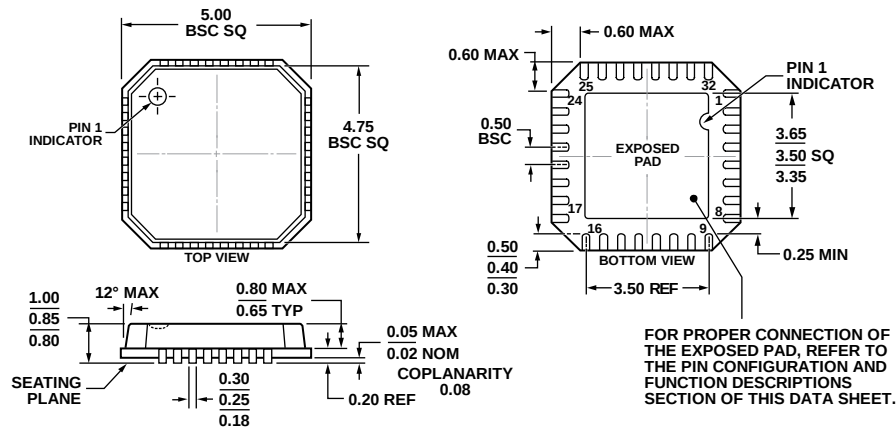
COMPLIANT TO JEDEC STANDARDS MO-220-VHHD-2 Figure 43. 32-Lead Lead Frame Chip Scale Package [LFCSP_VQ] 5 mm x 5 mm Body, Very Thin Quad (CP-32-4) Dimensions shown in millimeters
