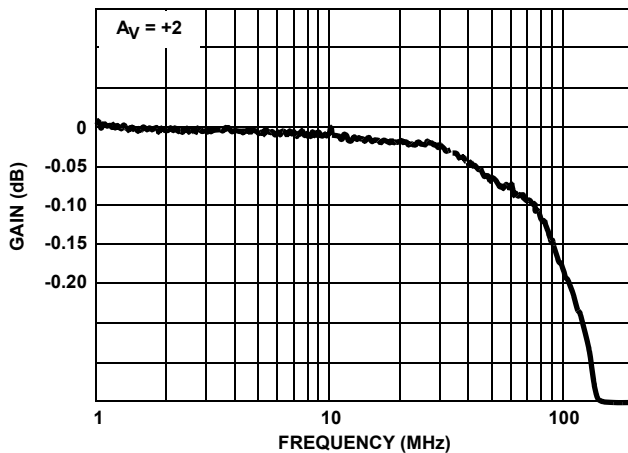
FIGURE 15. GAIN FLATNESS
