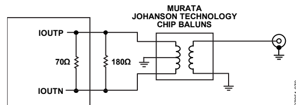
Figure 70. Lowest Cost and Size Configuration for Narrow RF Band Operation
