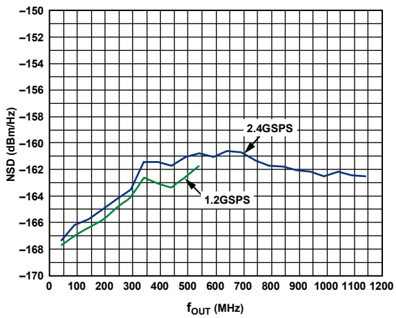
Figure 9. Single-Tone NSD over f_{OUT}
