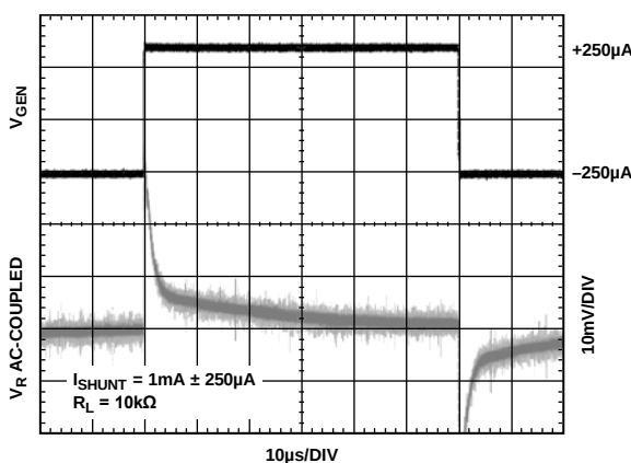
Figure 12. ADR5045 Transient Response
