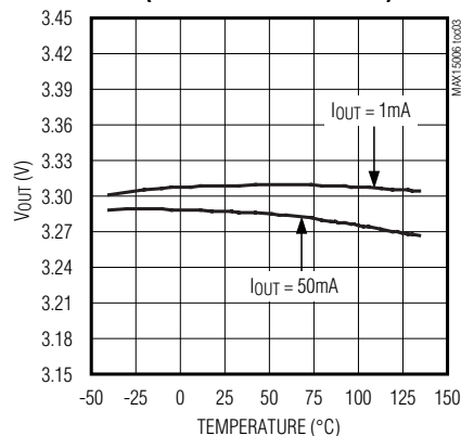
OUTPUT VOLTAGE vs. TEMPERATURE (MAX15006A/MAX15007A)
