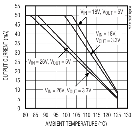
Figure 3a. Minimum Output Current vs. Ambient Temperature (6-Pin TDFN-EP)
