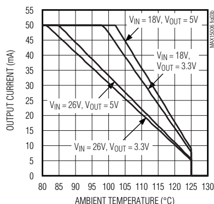
Figure 3b. Minimum Output Current vs. Ambient Temperature (8-Pin SO-EP)
