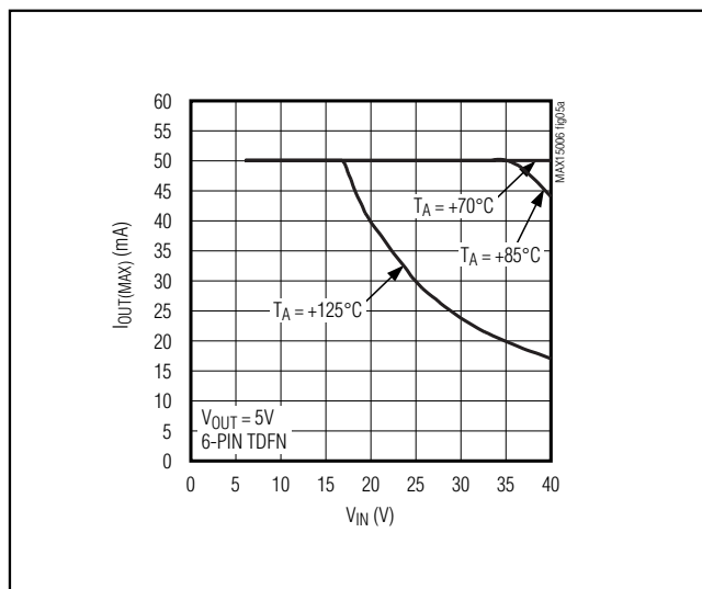
Figure 5a. Calculated Maximum Output Current vs. Input Voltage (6-Pin TDFN-EP)
