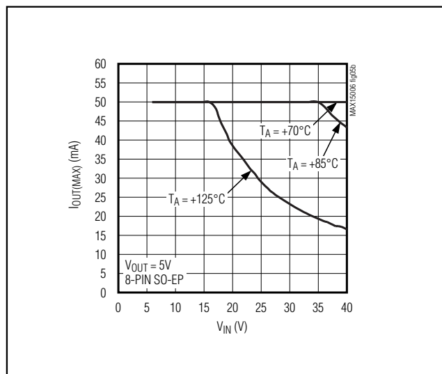
Figure 5b. Calculated Maximum Output Current vs. Input Voltage (8-Pin SO-EP)
