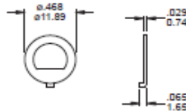
Locking ring supplied with B5 bushing
