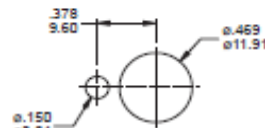
With standard locking ring.
