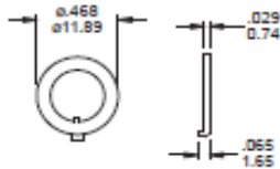
Locking ring supplied standard
