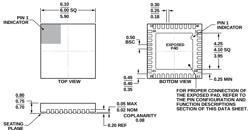
Figure 112. 40-Lead Lead Frame Chip Scale Package [LFCSP_WQ] 6 mm x 6 mm Body, Very Very Thin Quad (CP-40-9) Dimensions shown in millimeters
