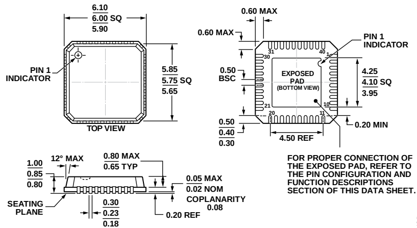
Figure 111. 40-Lead Lead Frame Chip Scale Package [LFCSP_VQ] 6 mm x 6 mm, Very Thin Quad (CP-40-1) Dimensions shown in millimeters
