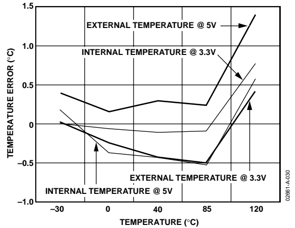
Figure 31. Temperature Error at 3.3V and 5V
