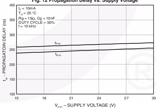
Fig. 12 Propagation Delay vs. Supply Voltage
