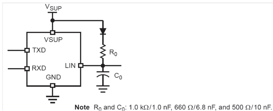
Figure 5. Test Circuit for Timing Measurements
