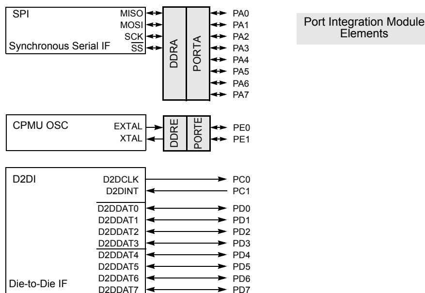
Figure 42. Block Diagram
