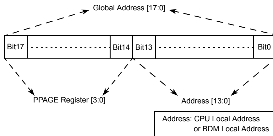
Figure 50. PAGE Address Mapping
