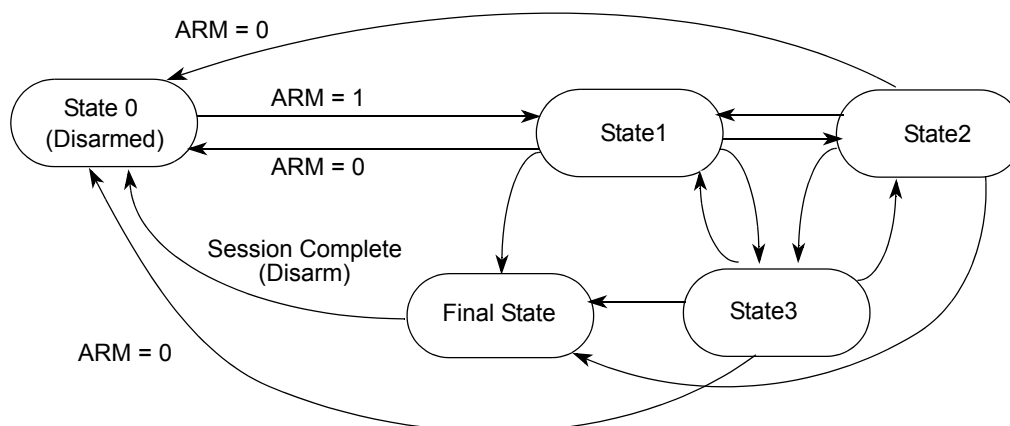
Figure 67. State Sequencer Diagram
