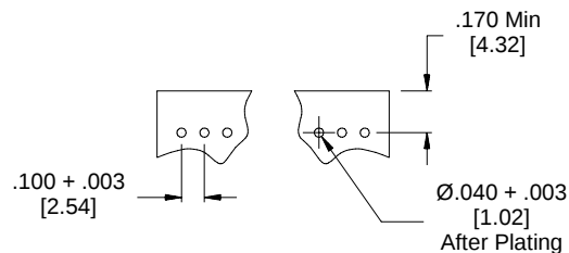
Right Angle Solder/Wrap Tails
