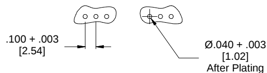
Straight Solder/Wrap Tails
