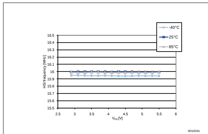
Figure 19: Typical HSI frequency variation vs V_{DD} @ 3 temperatures
