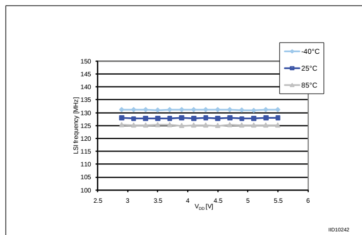
Figure 20: Typical LSI frequency variation vs V_{\text{DD}} @ 3 temperatures
