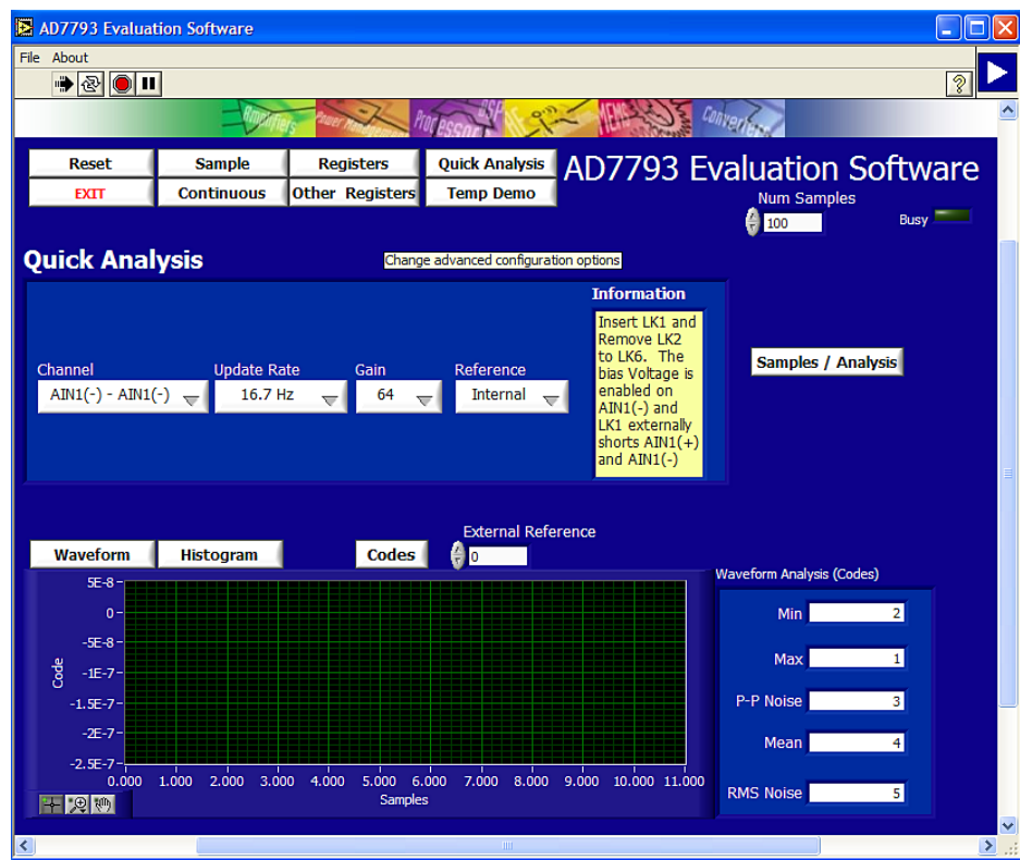
Figure 3. AD7793 Evaluation Software Main Window
