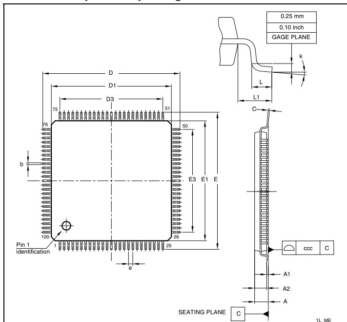
Figure 64. LQFP100, 14 x 14 mm 100-pin low-profile quad flat package outline (1)
