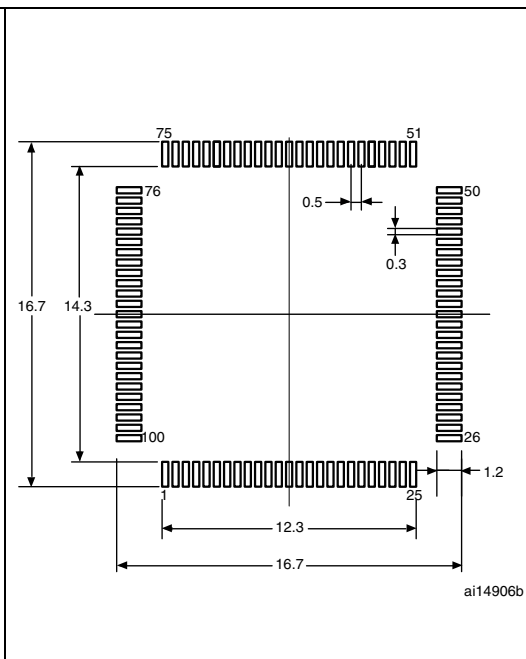
Figure 65. Recommended footprint (1)(2)
