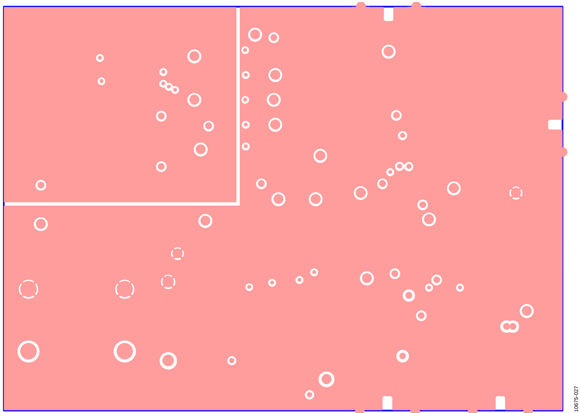
Figure 13. Layer 2 (Ground Plane)
