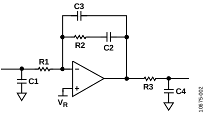
Figure 2. ADIsimPLL Filter
