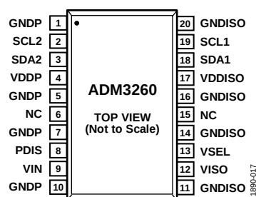
Figure 4. Pin Configuration
