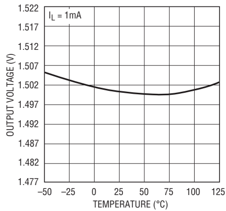
LT1965-1.5 Output Voltage
