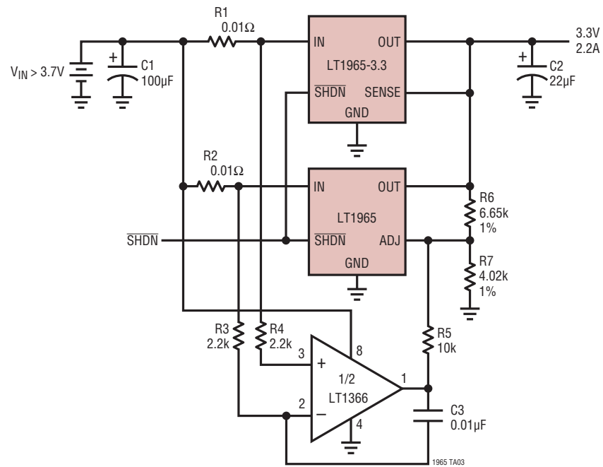
Paralleling of Regulators for Higher Output Current
