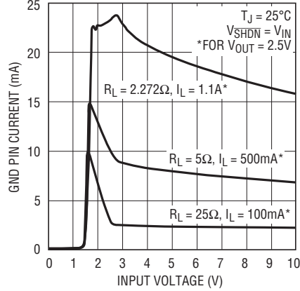
LT1965-2.5 GND Pin Current (Heavy Load)
