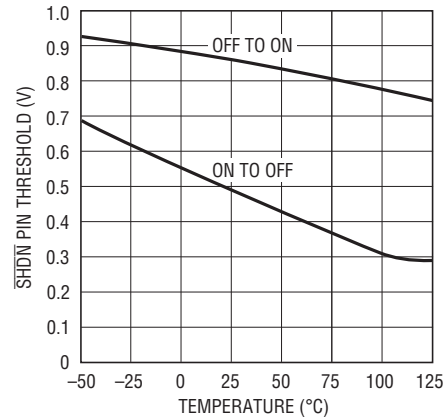
SHDN Pin Threshold
