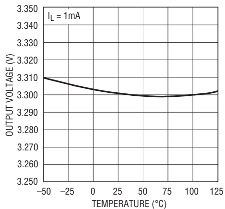
LT1965-3.3 Output Voltage
