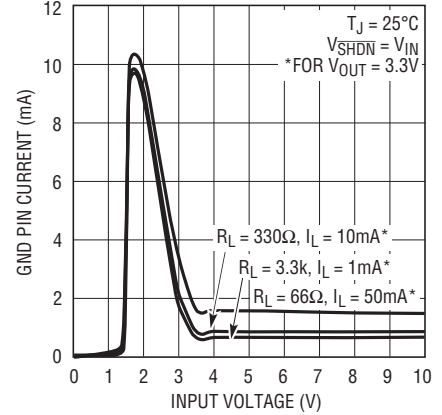
LT1965-3.3 GND Pin Current (Light Load)
