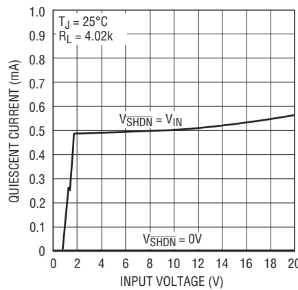
LT1965 Quiescent Current
