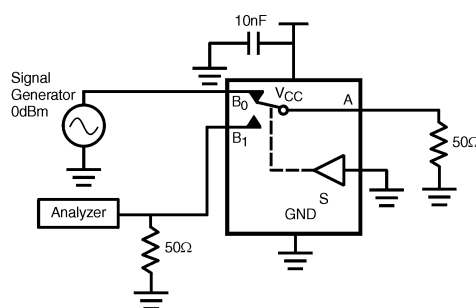
FIGURE 6. Crosstalk
