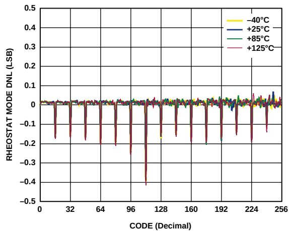
Figure 12. R-DNL vs. Code vs. Temperature, V_{DD} = 5\text{ V}
