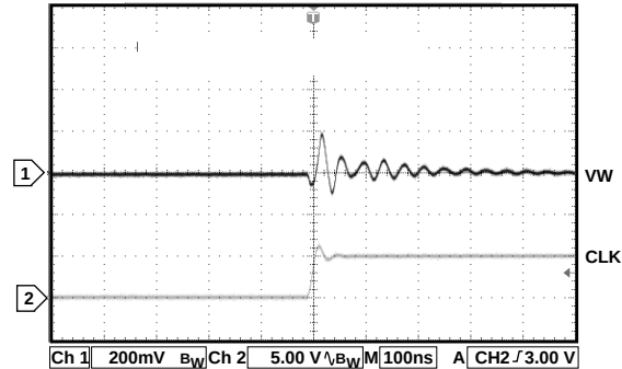
Figure 25. Digital Feedthrough
