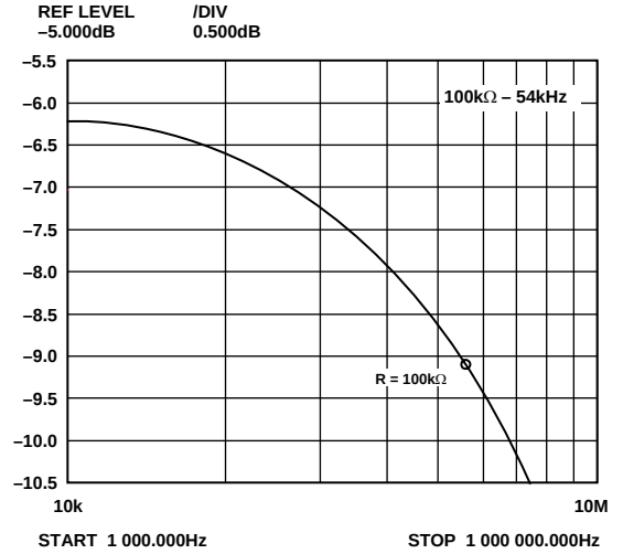
Figure 21. -3 dB Bandwidth @ Code = 0x80
