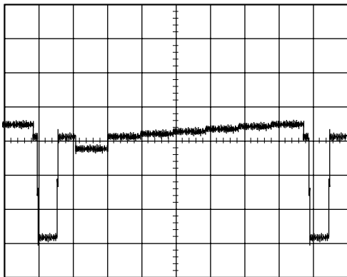
Figure 91. 525 p Black Bar (-35 mV, 0 mV, +7 mV, +14 mV, +21 mV, +28 mV, +35 mV)
