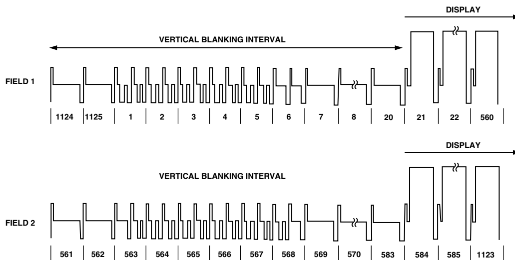
Figure 116. SMPTE274M (1080 i)
