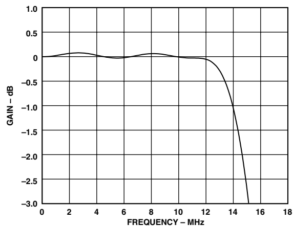
Figure 39. UV - HDTV 2 \times Oversampling Filter, Pass Band
