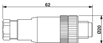
M12 x 1 plug, straight
