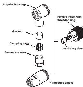
Male/Female M12
