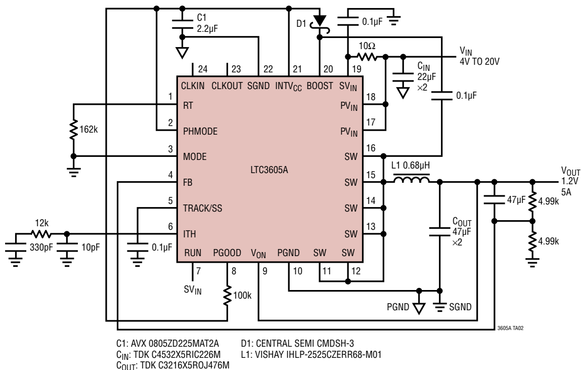
12V to 1.2V 1MHz Buck Regulator
