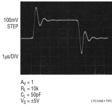
Small-Signal Transient Response
