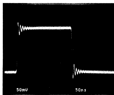
A_V = +2 , IN DEMO BOARD, C_L = 30pF WITH 10 \Omega ISOLATING RESISTOR
