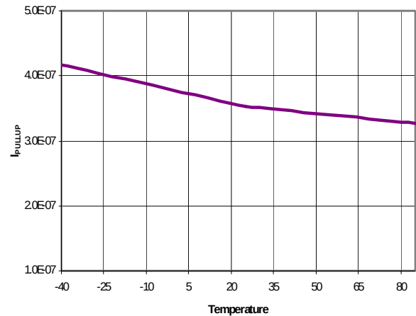
FIGURE 8. I PULL-UP vs TEMPERATURE AT V BAT = 1.8V
