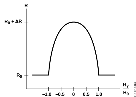
Figure 3. Permalloy Resistance vs. Magnetic Field
