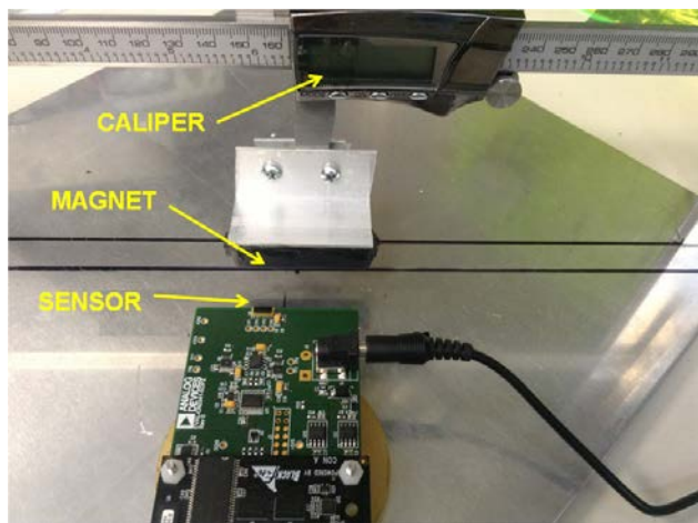
Figure 10. Photo of Bench Test Setup
