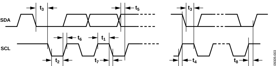
Figure 3. I²C Timing
