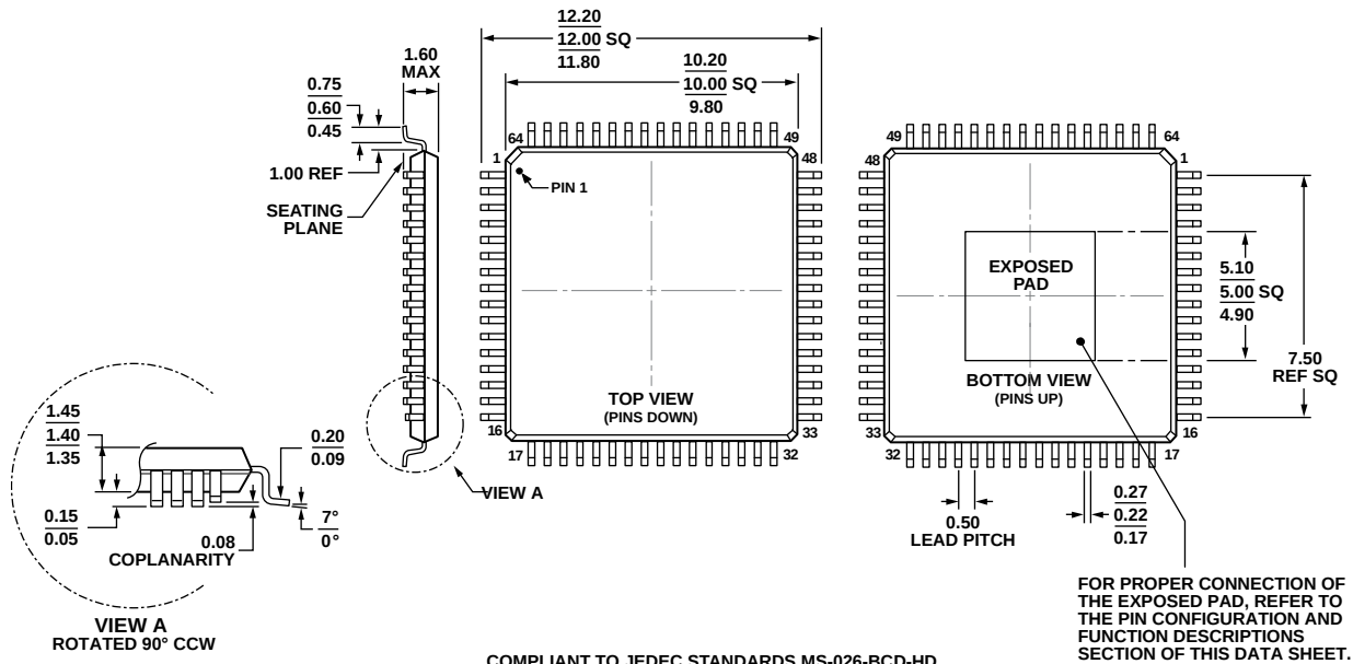
Figure 8. 64-Lead Low Profile Quad Flat Package (LQFP_EP)
