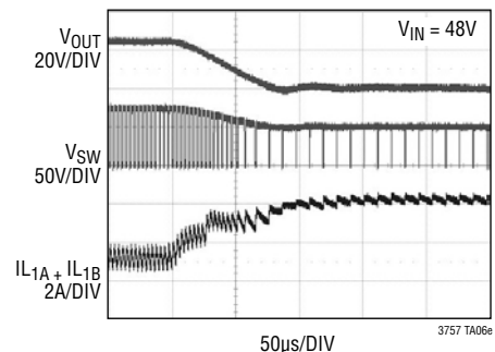
Frequency Foldback Waveforms When Output Short-Circuit
