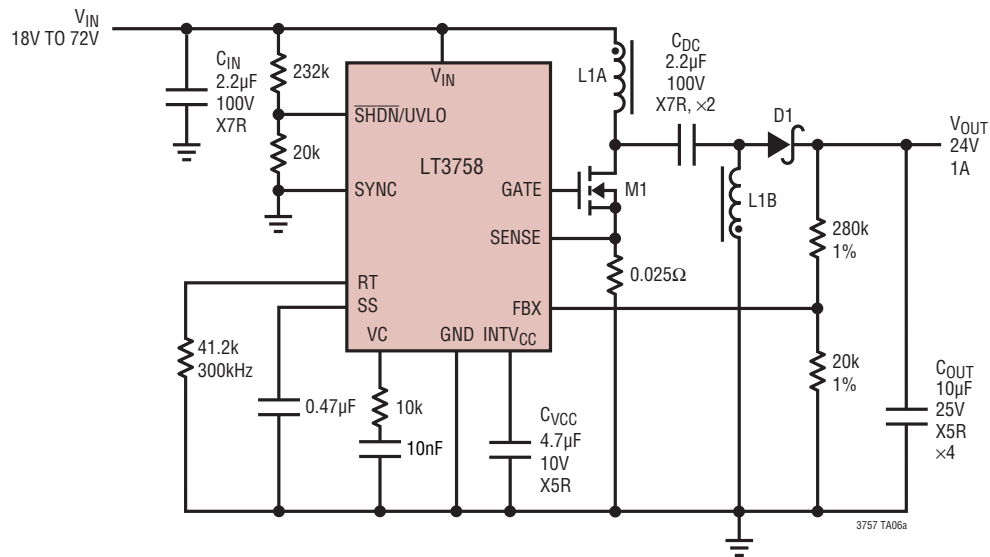
18V to 72V Input, 24V Output SEPIC Converter
