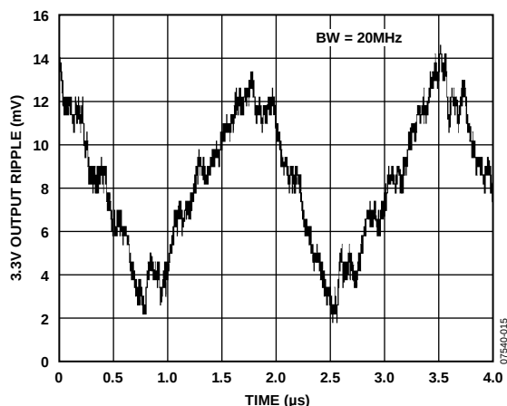
Figure 16. Typical Output Voltage Ripple at 90% Load, V_{ISO} = 3.3V
