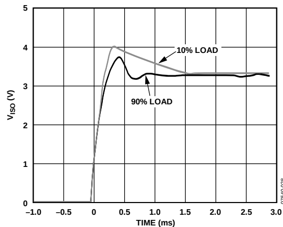
Figure 18. Typical Output Voltage Start-Up Transient at 10% and 90% Load, V_{ISO} = 3.3V
