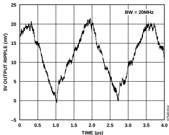
Figure 15. Typical Output Voltage Ripple at 90% Load, V_{ISO} = 5V
