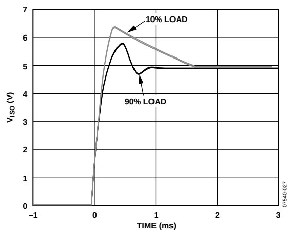
Figure 17. Typical Output Voltage Start-Up Transient at 10% and 90% Load, V_{ISO} = 5V
