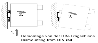
Snap-in Montage auf DIN-Tragschiene Snap-in mounting to DIN rail
