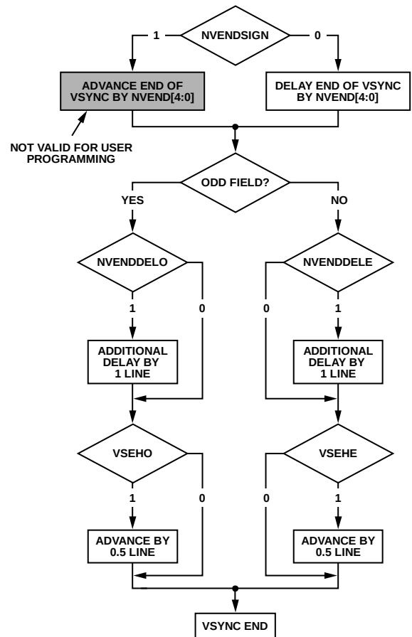
Figure 39. NTSC VSYNC End
