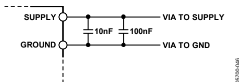
Figure 54. Recommended Power Supply Decoupling
