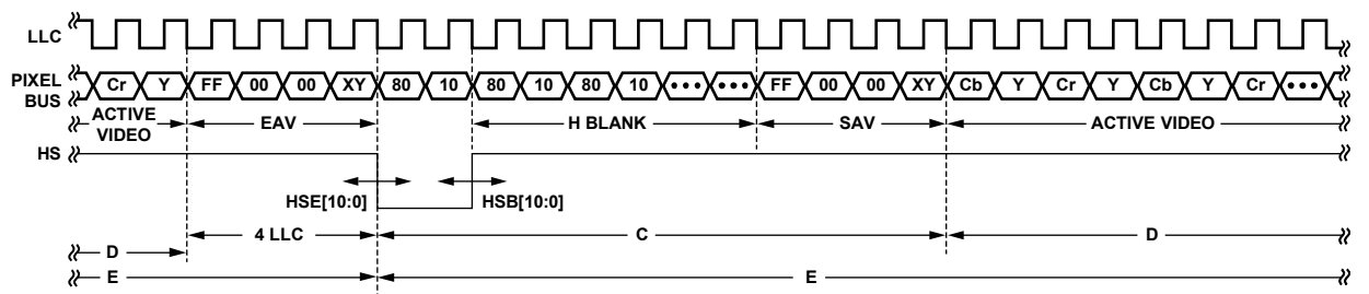
Figure 35. HS Timing
