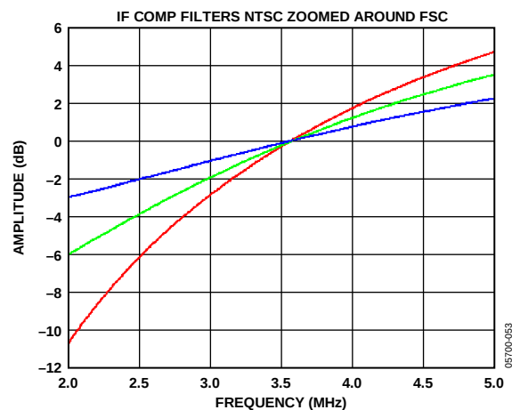
Figure 32. NTSC IF Filter Compensation
