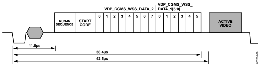
Figure 46. WSS Waveform
