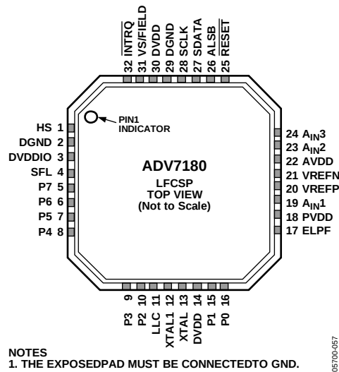
Figure 8. 32-Lead LFCSP Pin Configuration
