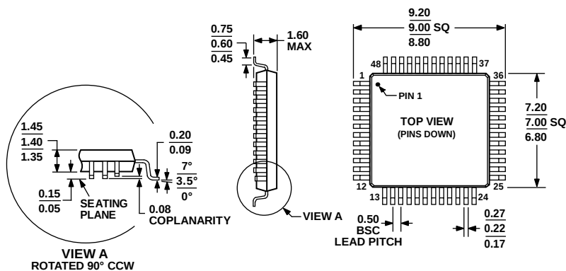
Figure 62. 48-Lead Low Profile Quad Flat Package [LQFP] 7 mm x 7 mm Body (ST-48)
