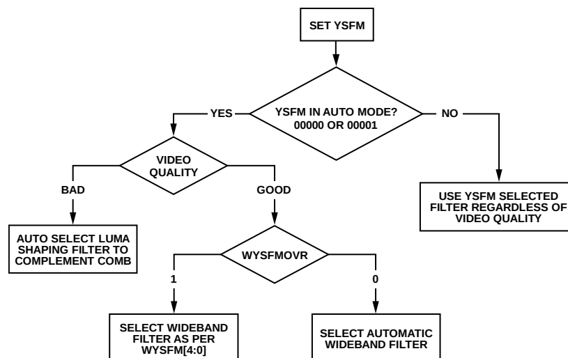
Figure 21. YFSM and WYSFM Control Flowchart
