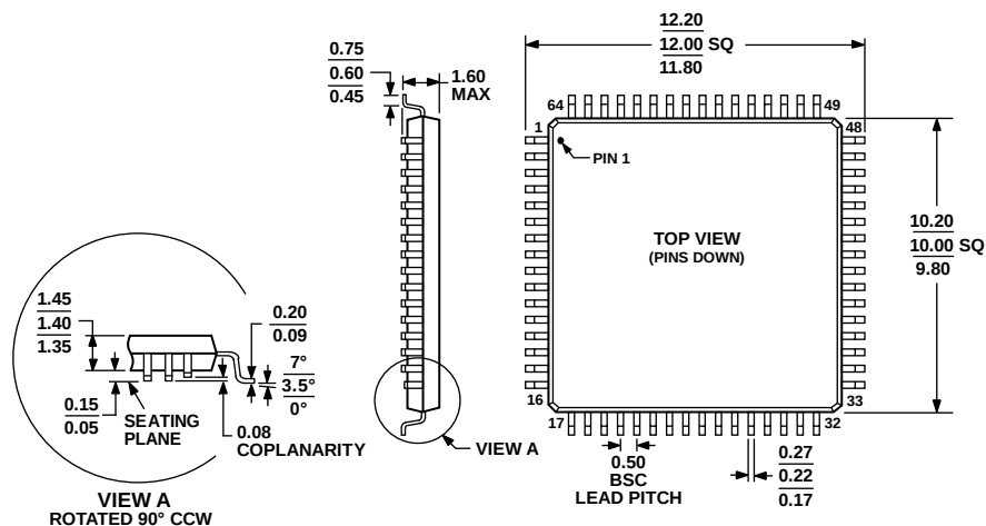
Figure 61. 64-Lead Low Profile Quad Flat Package [LQFP] 10 mm x 10 mm Body (ST-64-2)
