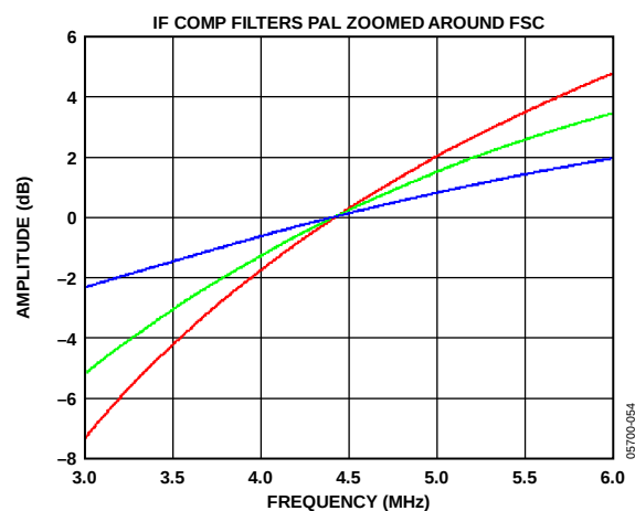
Figure 33. PAL IF Filter Compensation
