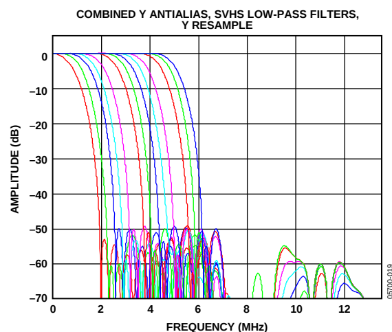
Figure 22. Y SVHS Combined Responses
