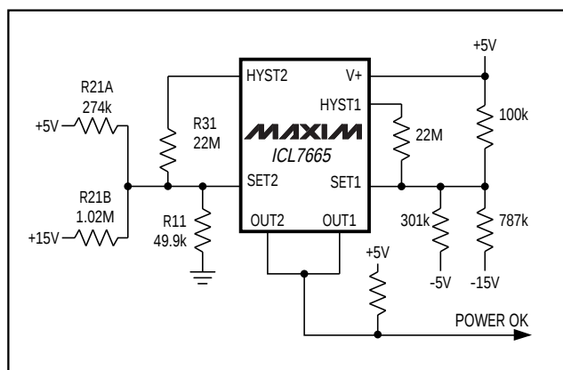
Figure 7. Multiple-Supply Fault Monitor
