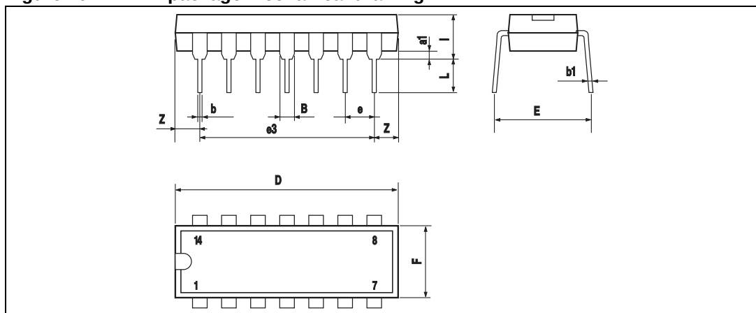
Figure 10. DIP14 package mechanical drawing
