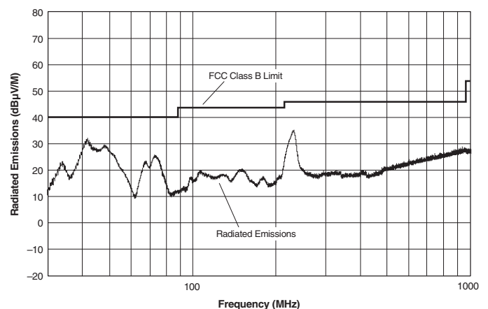
TWR-5/1000-12/125-D5A Radiated Emissions FCC Part 15 Class B, 3 Meters Converter Output = +5Vdc @ 950mA and \pm 12 Vdc @ \pm 114 mA
