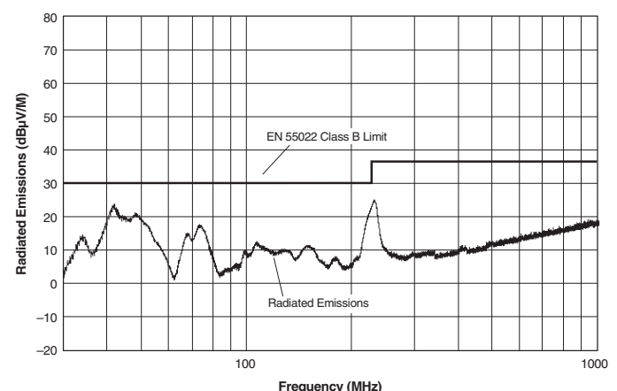
TWR-5/1000-12/125-D5A Radiated Emissions EN 55022 Class B, 10 Meters Converter Output = +5Vdc @ 950mA and \pm 12 Vdc @ \pm 114 mA
