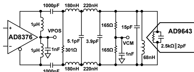
Figure 49. Differential Input Configuration Using the AD8376
