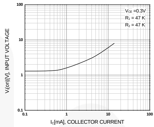
Figure 2. Input-On Voltage
